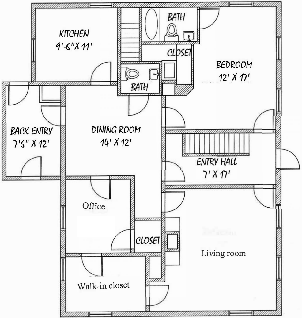
1 bedroom, 1st floor apartment in the William Gyles House Scaled drawing 1/8" = 1'0"
